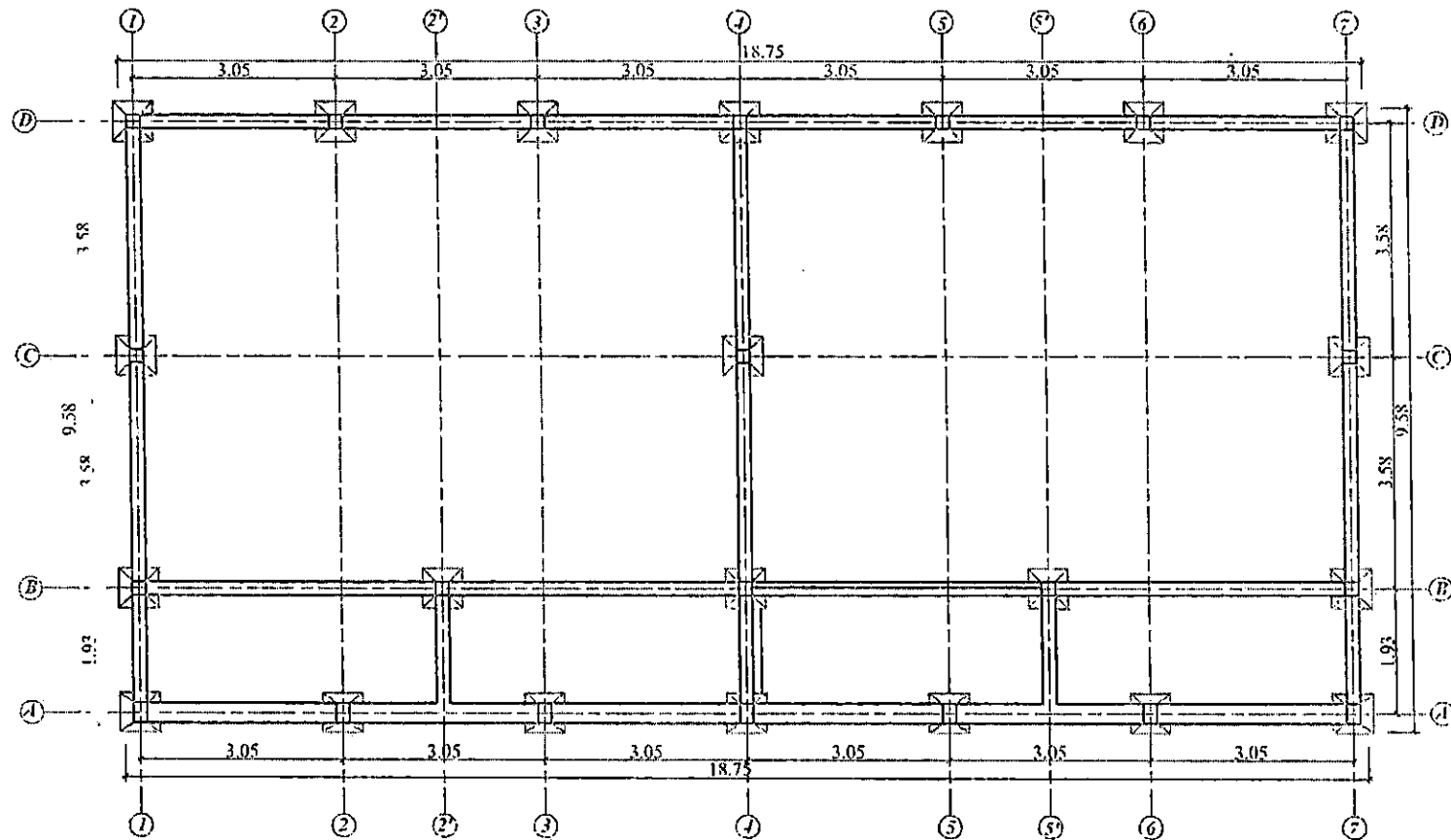
FOUNDATION PLAN
