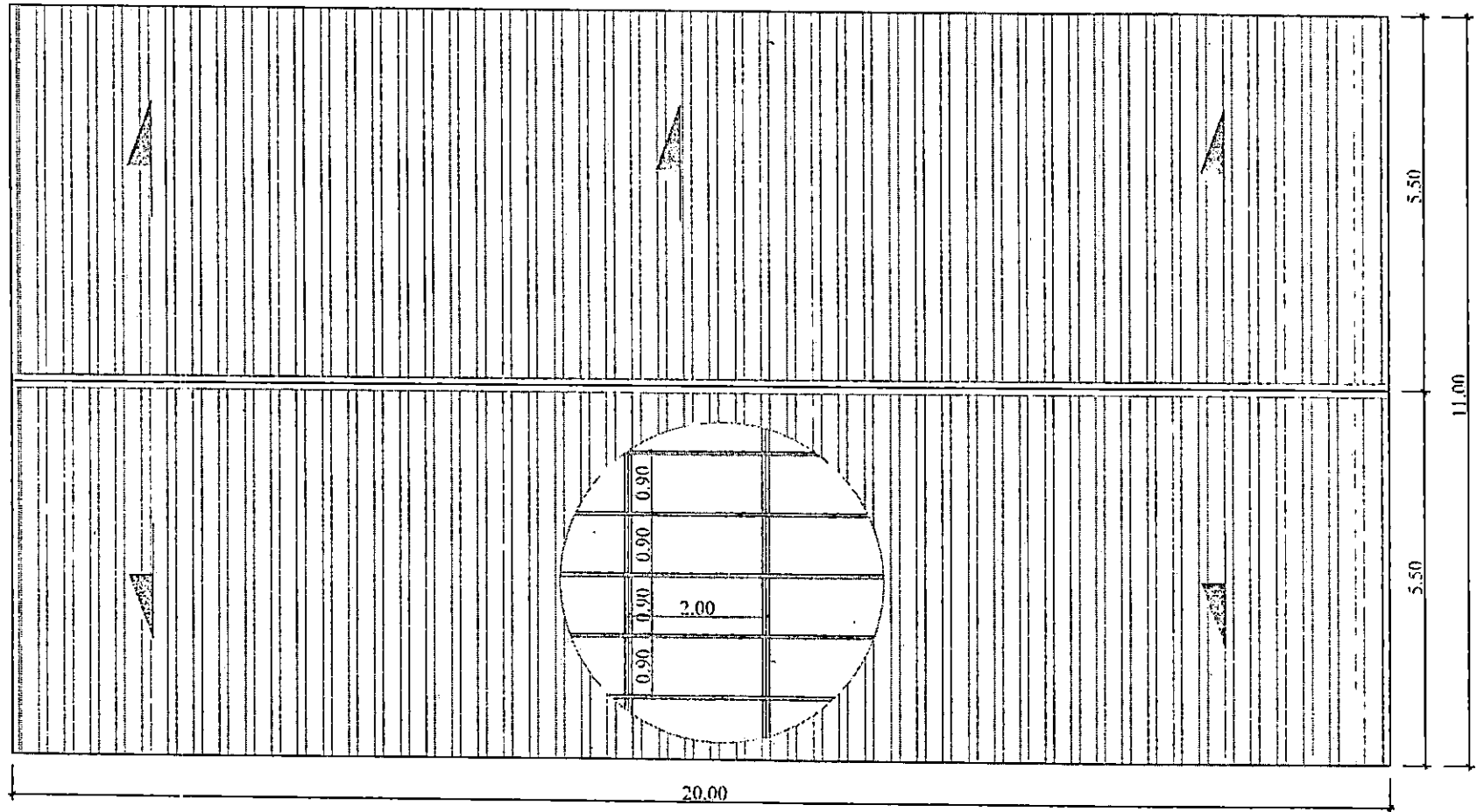
ROOF PLAN
