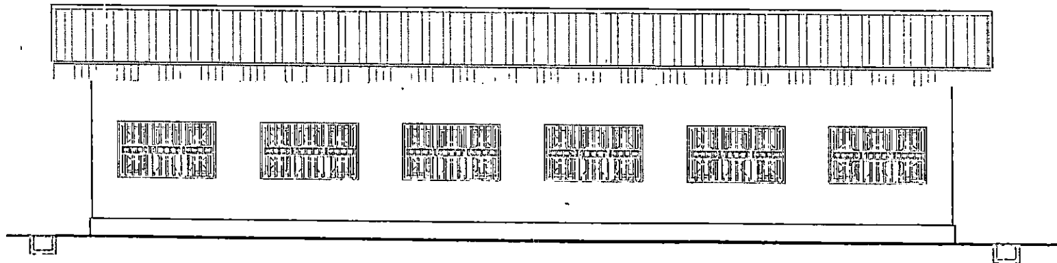
BACK ELEVATION
