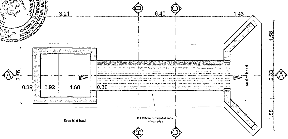
PLAN OF METAL RING CULVERT
