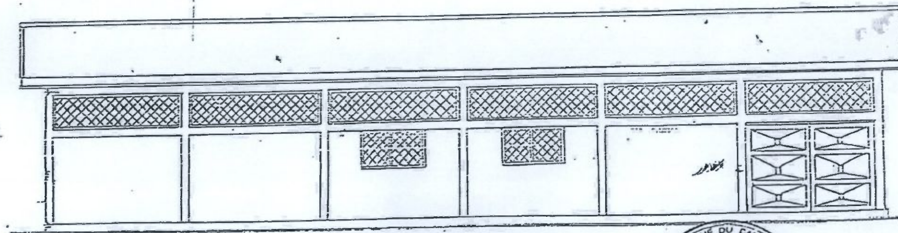
FRONT ELEVATION
