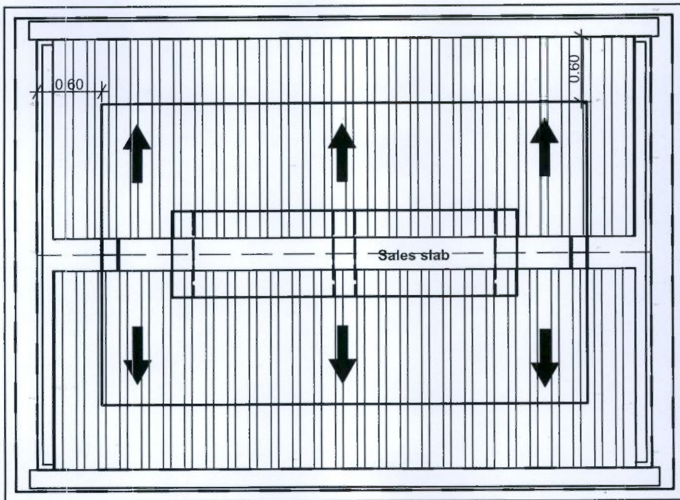
Roof Plan
