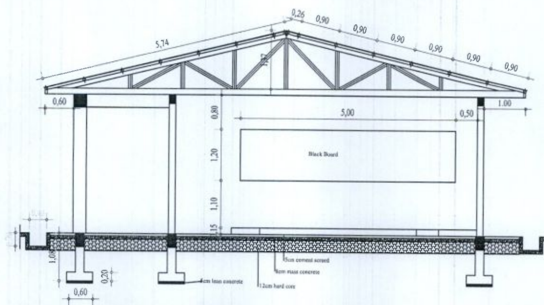
SECTION C-C
