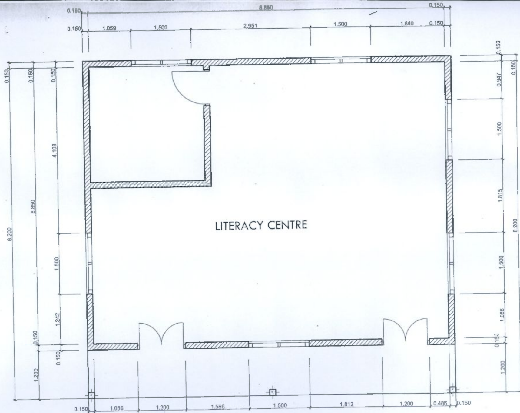
GROUND PLAN
