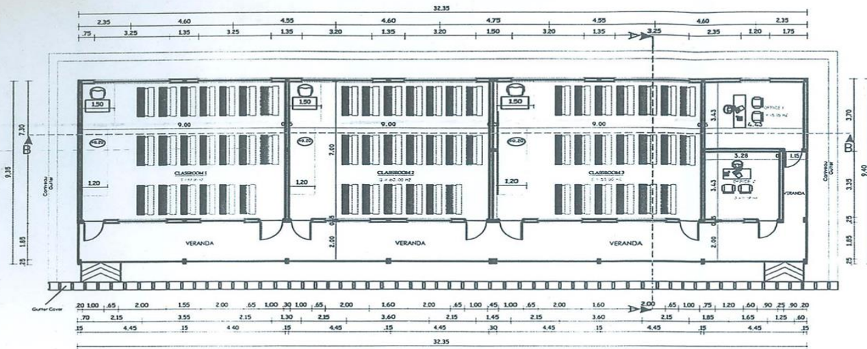
PLAN DE DISTRIBUTION DISTRIBUTION PLAN
